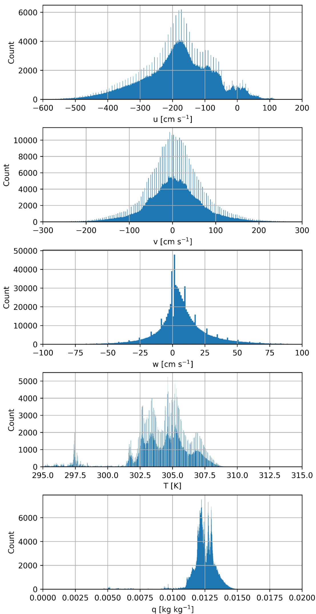
Figure S1. Histograms of horizontal wind speed u and v , vertical wind speed w , Temperature and specific humidity during 11 September 2023 as measured by the eddy-covariance system.
