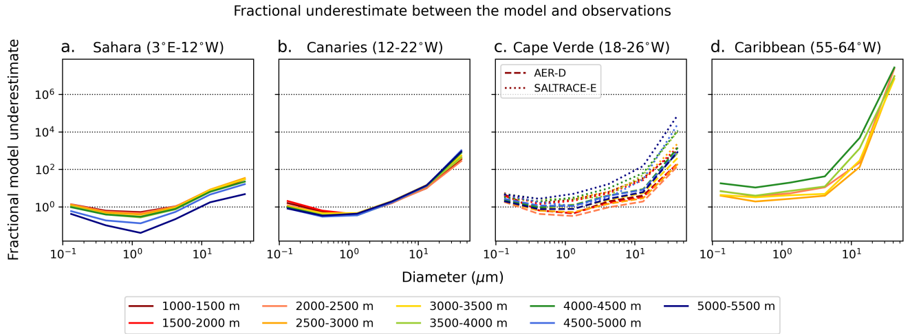
Figure 5. Fractional underestimate of the volume size distribution between the observations and model. The vertically-resolved difference is shown at the Sahara (a) and Canaries (b), using Fennec observational data, at Cape Verde (c) using AER-D (dashed lines) and SALTRACE-E (dotted lines) data and at the Caribbean (d) using SALTRACE-W data.
