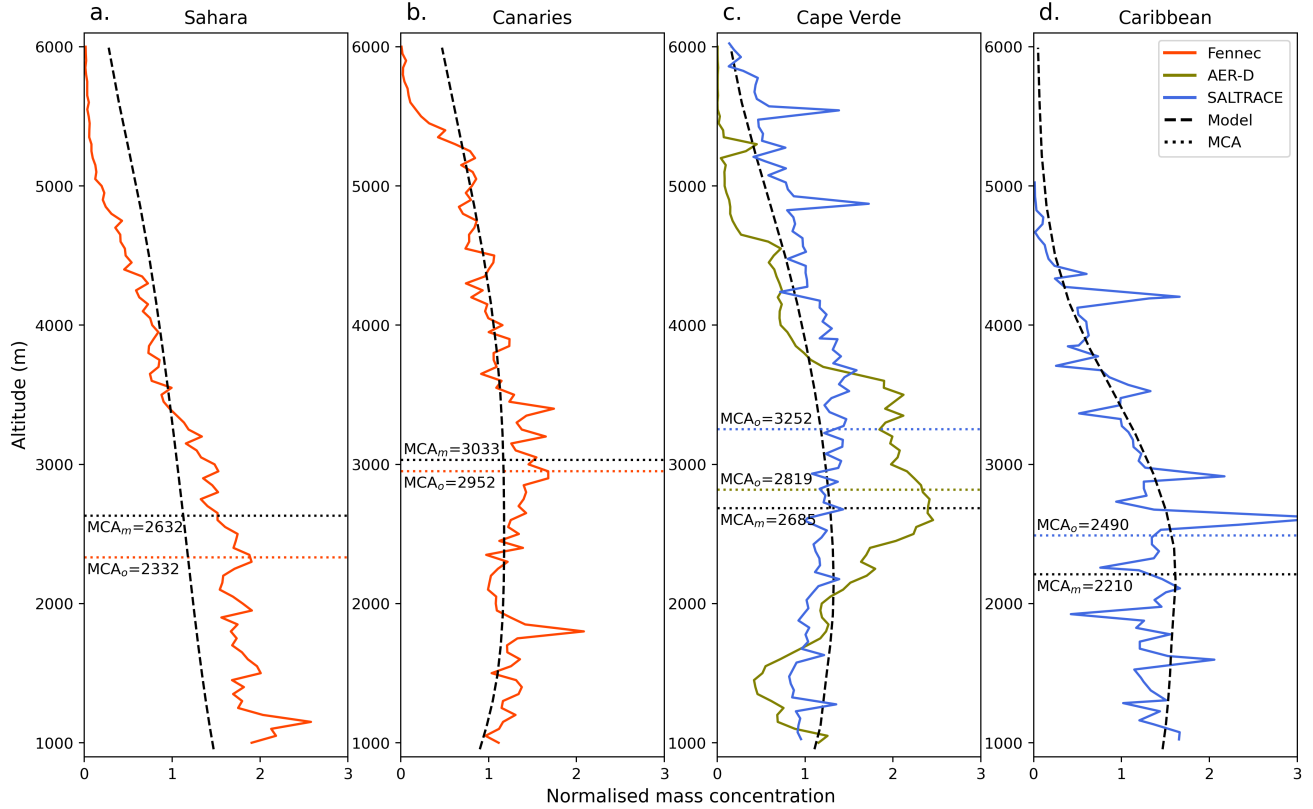
Figure 2. Normalised observed (coloured solid line) and modelled (black dashed line) total dust mass concentration profile and dust mass centroid altitude (MCA; dotted horizontal lines in metres) between 1-6 km. MCA_o and MCA_m respectively represent the observed and modelled MCA values. Plots show all four observed locations: Sahara (a), Canaries (b), Cape Verde (c; AER-D and SALTRACE-E) and Caribbean (d; SALTRACE-W) from the Fennec (orange), AER-D (green) and SALTRACE (blue) campaigns. Data has been normalised by the mean profile concentration between 1-6 km altitude.
