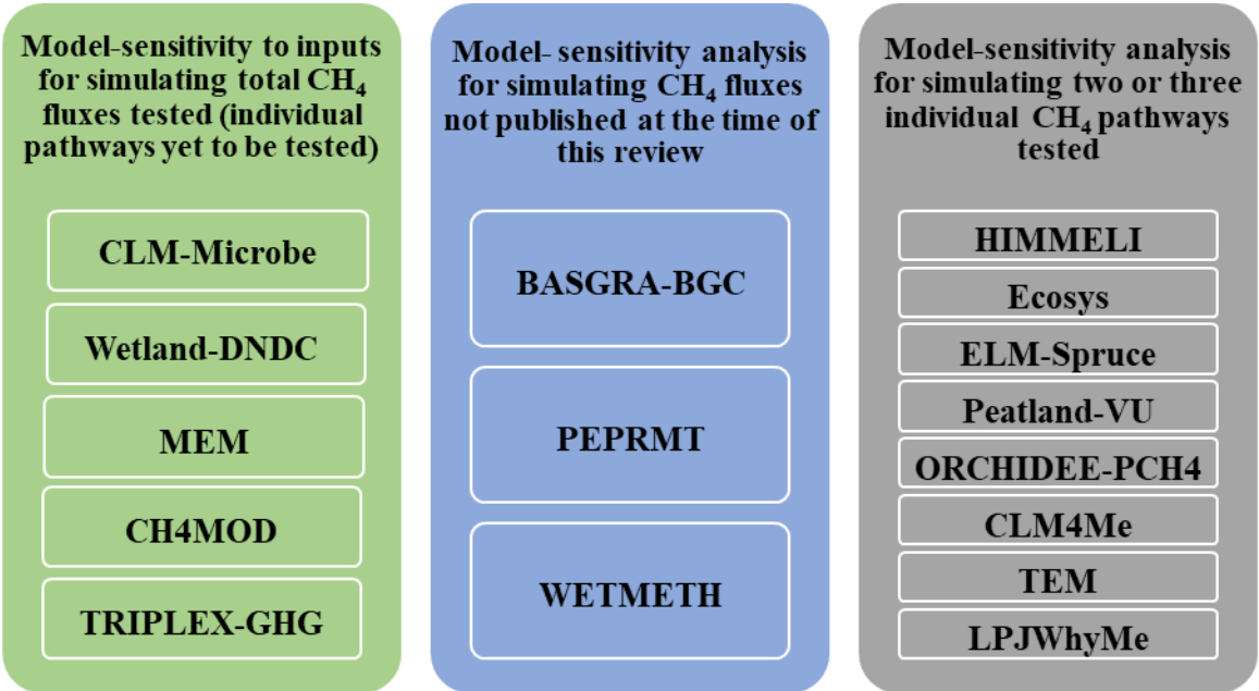
Figure 5. Reviewed peatland or wetland models distinguished into three categories shown above. Note: this figure reflects the information relevant to this review only and at the time when this review was conducted.
