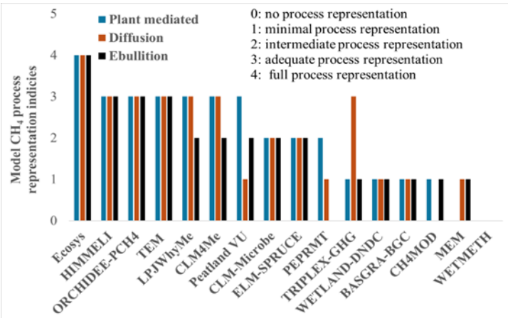
Figure 4. CH 4 process representation indices of plant-mediated transport, diffusion and ebullition. Note: the definition of the process representation indices is described in detail in section 2.2.
