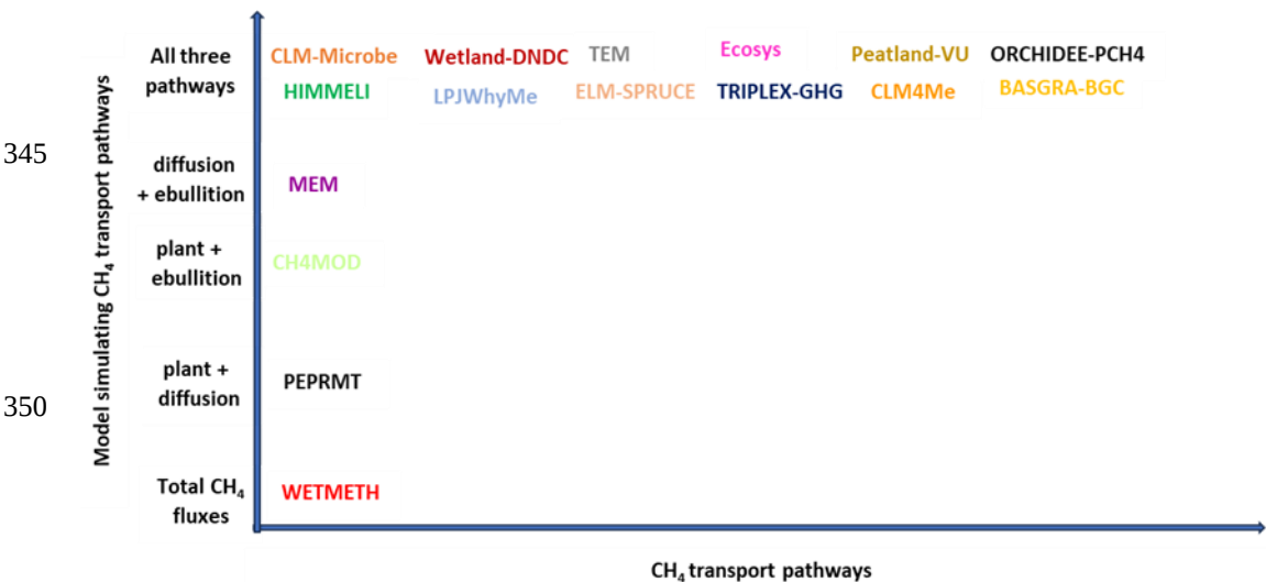
Figure 2. Reviewed peatland or wetlands models simulating CH 4 transport pathways. Each model has its own unique colour for easy identification. The + sign means model simulates both mentioned CH 4 transport pathways.
