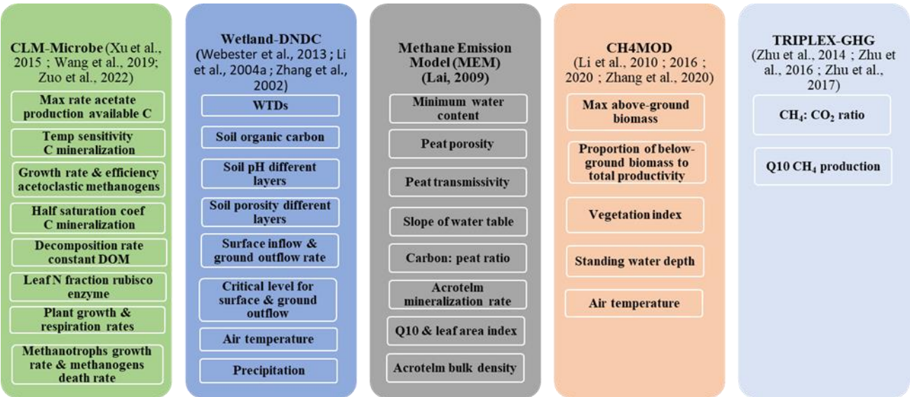
Figure 6. Critical inputs in each model impacting total CH 4 flux predictions.
