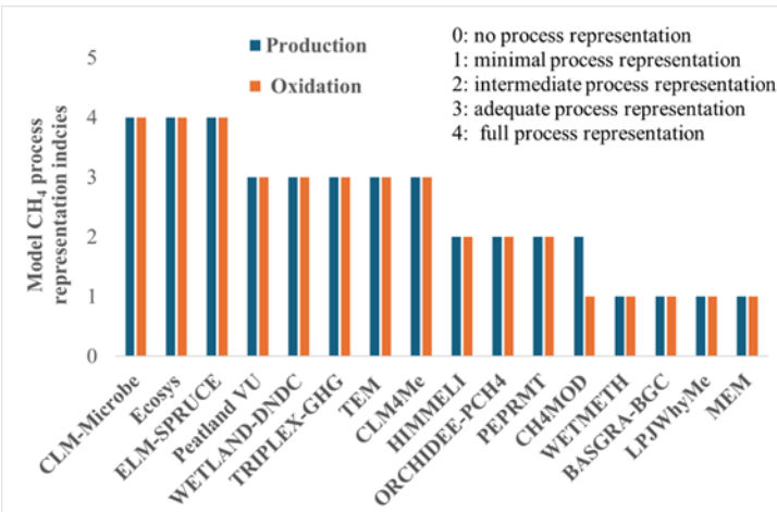
Figure 3. CH 4 process representation indices of production and oxidation. Note: the definition of the process representation indices is described in detail in section 2.2.
