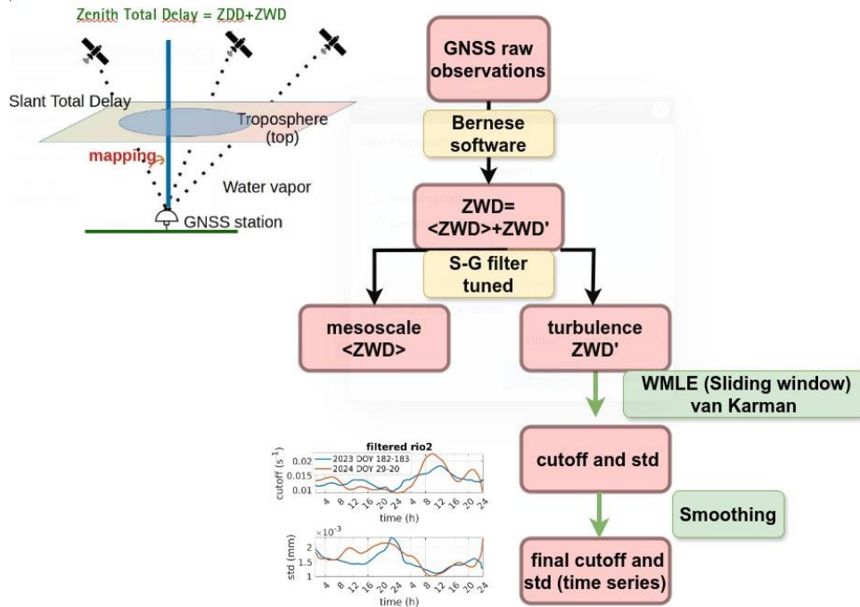
Figure 2. Flowchart summarizing the methodology from the processing of raw GNSS observations to the time series of turbulent parameters \alpha et \sigma . The small figures are for illustration only.
