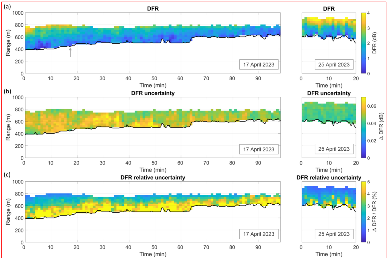
Figure 3: (a) Dual frequency reflectivity ratio, (b) associated uncertainty, and (c) relative uncertainty for the observation periods. The arrow at minute 18 in (a) points at the profile used in Fig. 4.
