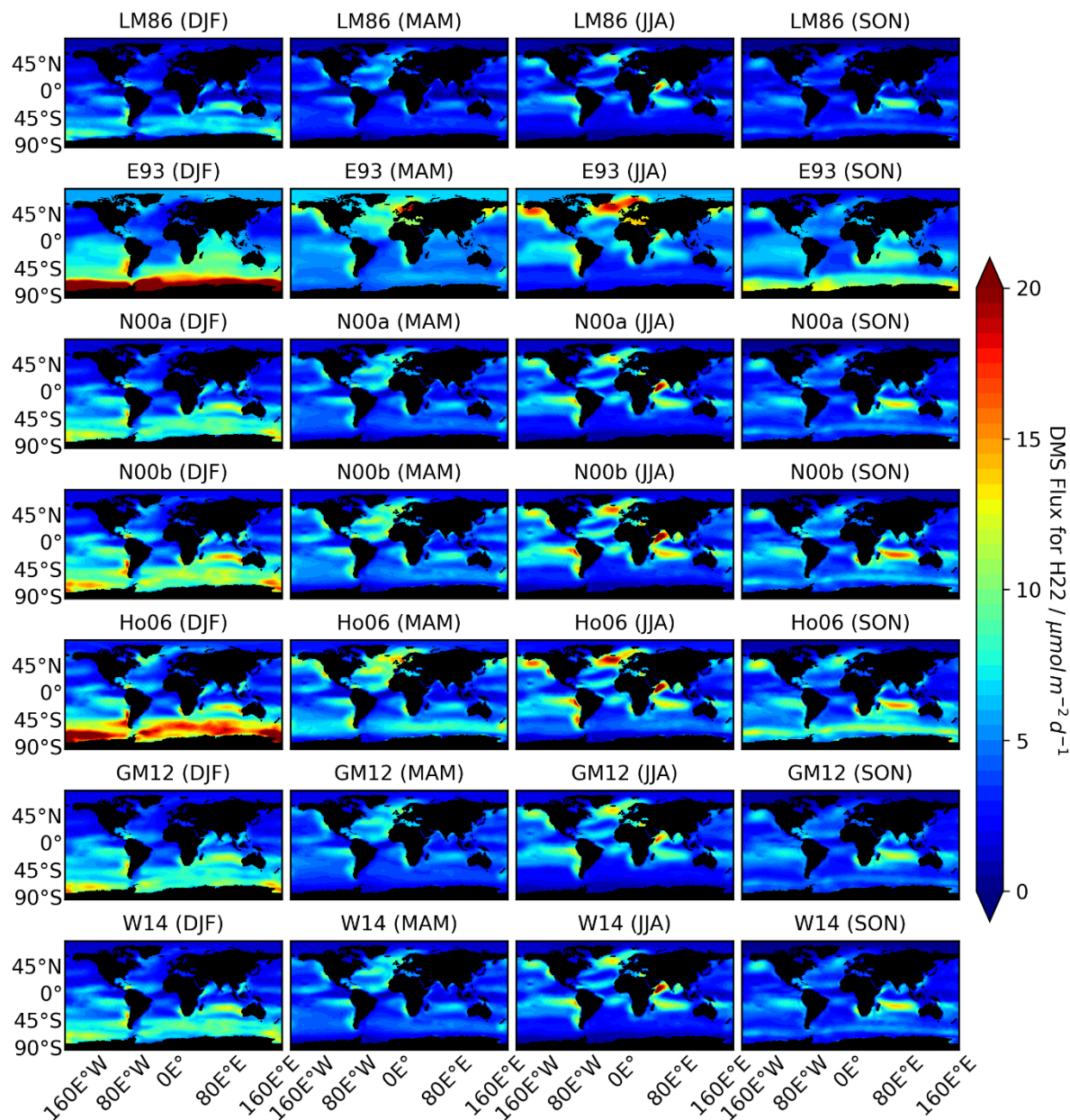
Figure 1: DMS fluxes estimated using the seven parameterizations for different seasons using the H22 climatology. The geographical pattern is similar in all the estimates, although the absolute values differ according to the parameterization chosen. In June-July-August (JJA) , a maximum flux of 33.75 \mu\text{mol m}^{-2} \text{d}^{-1} is calculated in Indian ocean near Somalia with N00b. In December-January-February (DJF) , a maximum flux of 45.82 \mu\text{mol m}^{-2} \text{d}^{-1} is calculated in Weddell Sea region with E93.
