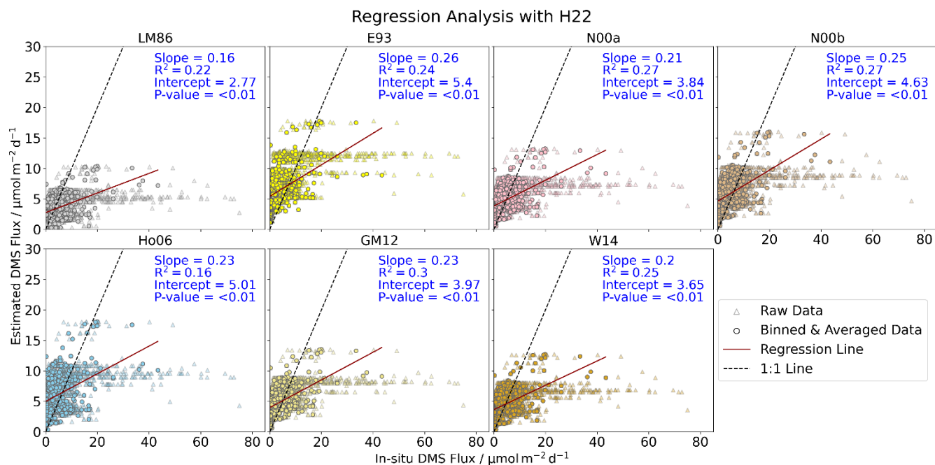
Figure 4: Comparison of in situ and estimated DMS fluxes (using H22) with the different parameterizations. Here, the regression analysis is done with binned and averaged in situ data at 1^\circ \times 1^\circ resolution, as the flux climatologies are also at the same resolution. The analysis shows that flux calculations result in higher fluxes than observations at low levels ( < 20 \mu\text{mol m}^{-2} \text{d}^{-1} ) and lower fluxes than observations at higher levels ( > 20 \mu\text{mol m}^{-2} \text{d}^{-1} ), which indicates that flux parametrization methods fail to represent the range accurately. The black dash line is the 1:1 representation between in situ and the estimated DMS flux points, and the dark red line is the regression line. A list of the in situ observations used for the comparison is given in Table S1.
