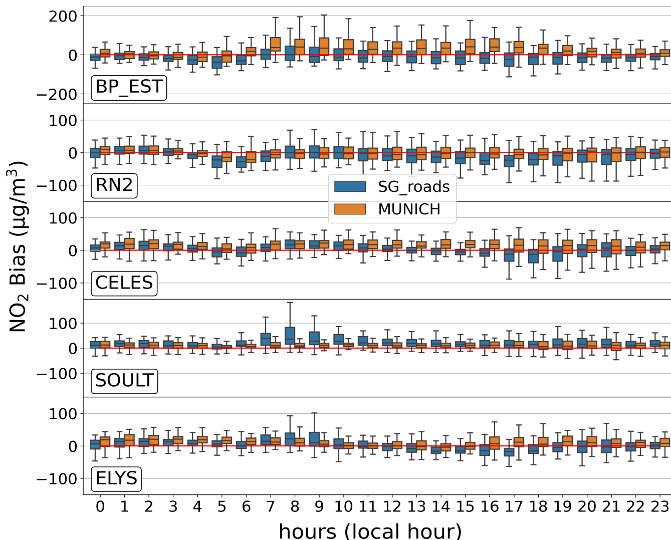
Figure D2. Daily profiles of the bias (in \mu\text{g.m}^{-3} ) between observed and simulated concentrations for the period of February-March 2014, for \text{NO}_2 concentrations.
