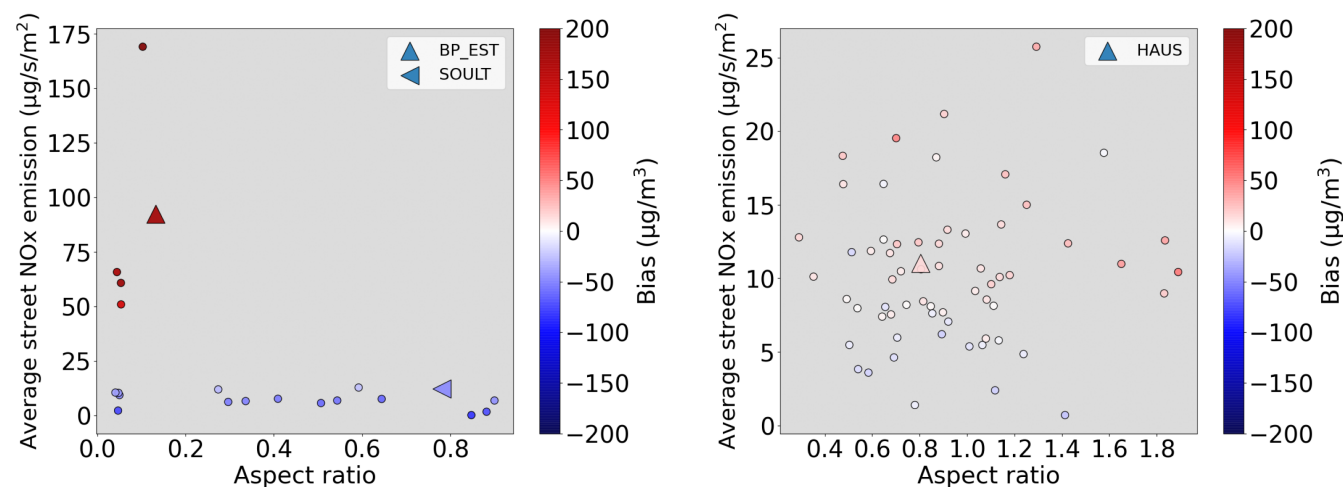
Figure 7. Bias between MUNICH and the Subgrid method for \text{NO}_x , as a function of the \alpha_r (X axis) and the average emissions of MUNICH (Y axis, in \mu\text{g}\cdot\text{s}^{-1}\cdot\text{m}^{-2} ) of all the streets (point) of a cell, over February and March 2014. The left panel shows the results for the cell containing stations BP_EST and SOULT, the right one for the cell containing HAUS.
