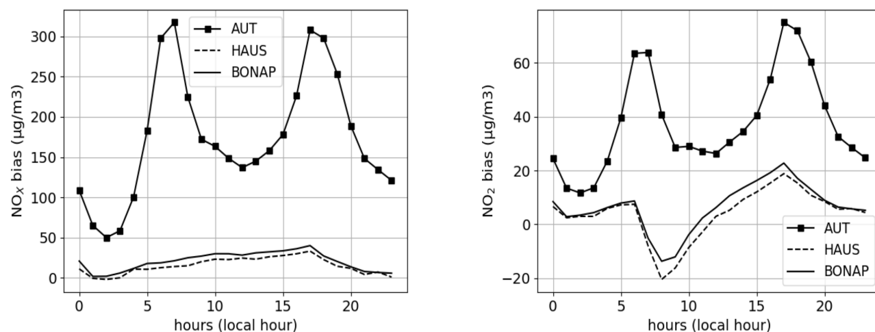
Figure 10. Daily profiles of the bias (in \mu\text{g.m}^{-3} ) between MUNICH and Subgrid simulations over the period of February-March 2014, for \text{NO}_x and \text{NO}_2 concentrations.
