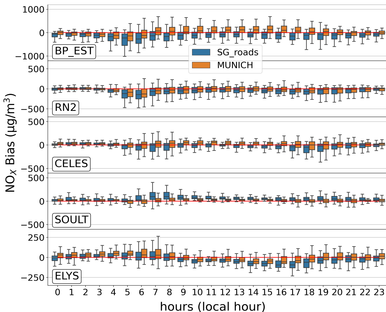
Figure D1. Daily profiles of the bias (in \mu\text{g.m}^{-3} ) between observed and simulated concentrations for the period of February-March 2014, for \text{NO}_x concentrations.
