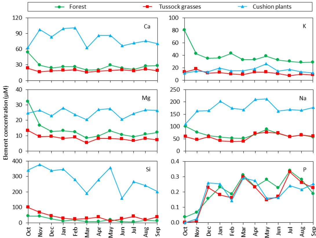
Figure 7: Temporal variation in soil solute concentrations under forest (n=7), tussock grasses (n=15) and cushion plants (n=9). The mean monthly values for the period October 2012 till September 2013 are plotted in the graphs. Even after a 2-month equilibration period, we cannot entirely exclude that the first cation concentration measurements under forest (October 2012) are higher-than-expected due to incomplete stabilization of the lysimeters after installation (e.g. preferential flow because of lysimeter insertion).
