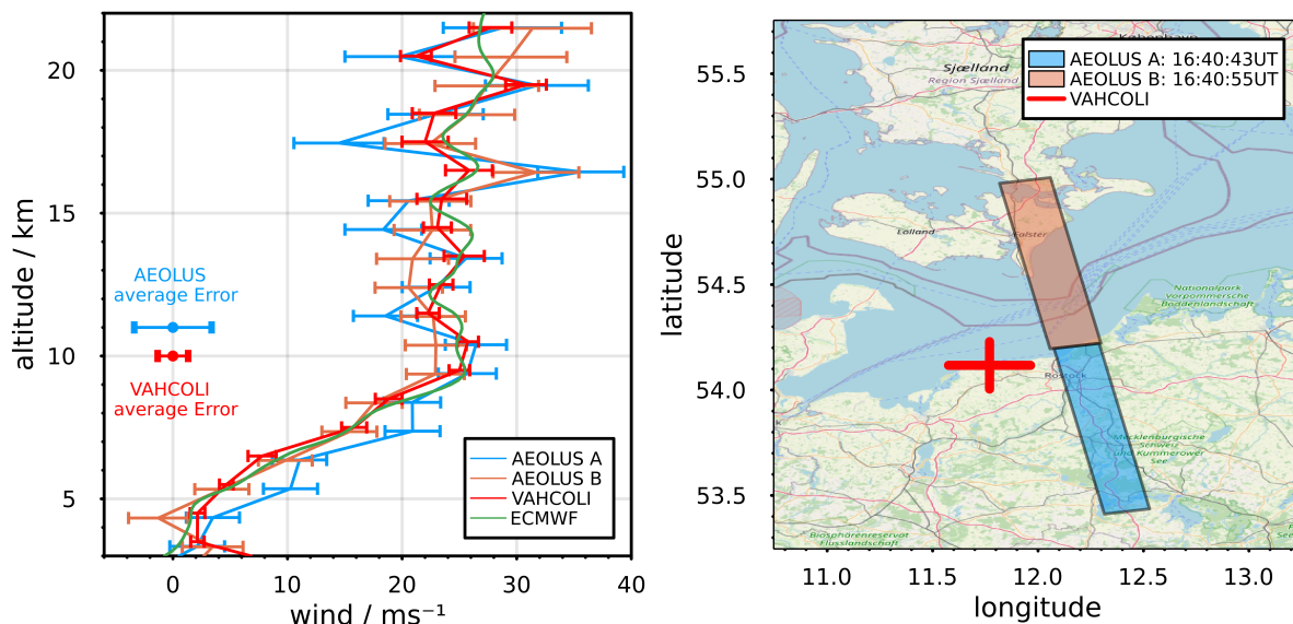
Figure 11. left: Comparison of the winds measured by Aeolus (blue and orange lines) and the VAHCOLI 1 lidar system (red lines) together with the winds from ECMWF (green line). For winds from VAHCOLI and ECMWF the meridional, zonal and vertical components have been combined and projected on to the horizontal line of sight (HLOS) of Aeolus. The difference of the lidar measurement and the B profile from Aeolus is -0.12 \pm 3.31 \text{ m s}^{-1} on average, with the best agreement below 15 km. Additionally the average error for the VAHCOLI winds ( 1.3 \text{ m s}^{-1} , red) and the Aeolus winds ( 3.3 \text{ m s}^{-1} , blue) are marked. right: Map showing the integration areas for the two Aeolus profiles (orange & blue boxes) together with the VAHCOLI beams (red lines) up to a height of 25 km. (data: (© OpenStreetMap contributors, 2017))
