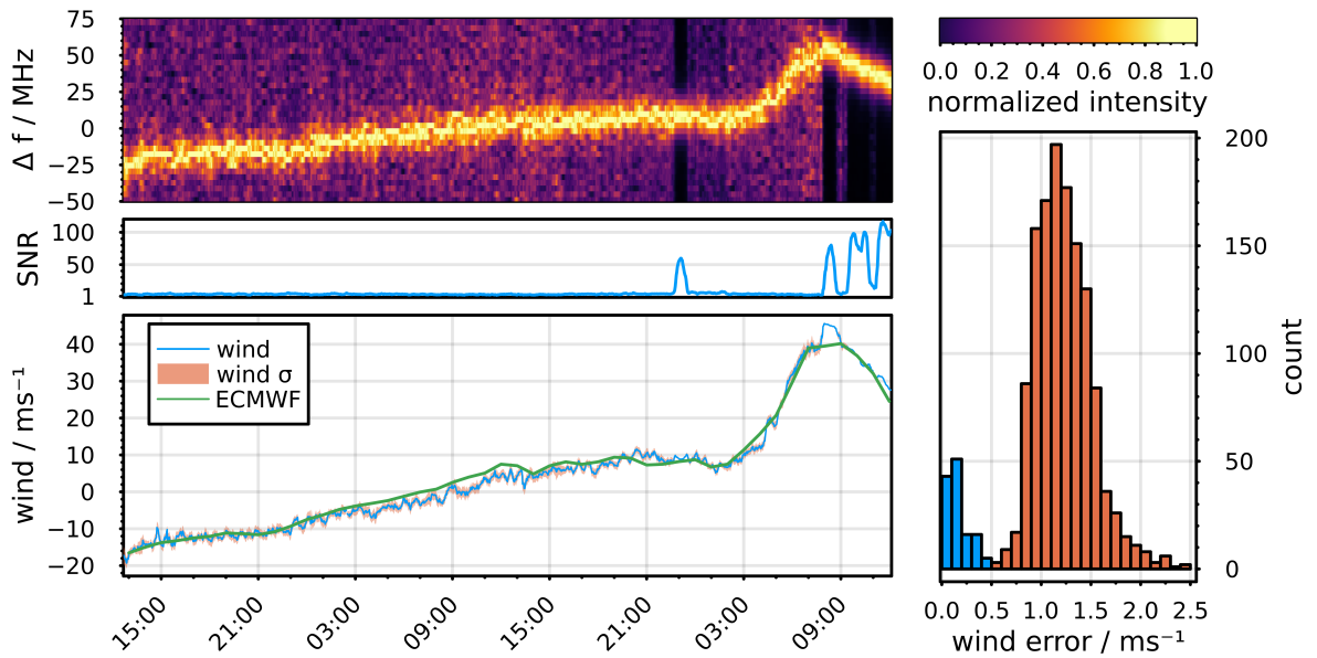
Figure 4. Connection between measured spectra, calculated wind and wind error. top left: Example of an atmospheric spectrum measured between the 16th and 18th of December 2022 with the north-facing telescope integrated from 9.25 km to 10.25 km, a gridded time resolution of 2 minutes and an integration time of 20 minutes. The purple and black regions in the spectrum plot represent the lidar background. The black corresponds to the cirrus clouds seen in Fig. 3 which result in a higher SNR value. centre left: Signal-to-noise ratio (SNR) calculated from the spectrum above. top left: Calculated lidar average wind speed (blue) together with the wind error estimate (orange ribbon), which most of the time at line strength of the wind speed. The corresponding ECMWF-IFS wind time series is shown for reference (green). A significant deviation of the measured wind and the ECMWF wind is visible at the 18th December around 8:00 UT, probably caused by the much higher smoothing in ECMWF. bottom right: Histogram of the error estimate for the wind from measurements with high (blue) and low (orange) aerosol loading.
