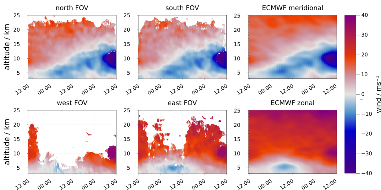
Figure 6. Horizontal winds measured between December 16th 12:00 UT and 18th 12:00 UT in the north/south/west/east fields of view (see plot titles) using a vertical integration of 1000 m and an integration time of 2 hours. The corresponding meridional and zonal winds from ECMWF are shown in the two right-most panels. The integration window was shifted in 100 m and 2-minute steps. Winds with a line of sight wind error of more than 2 \text{ m s}^{-1} are masked. The line of sight winds of the tilted telescopes are converted to zonal and meridional winds. In the meridional winds a clear transition around the tropopause from mainly southward winds at the beginning of the measurement to strong northward winds at the end is visible. The lower signal strength in the zonal FOVs causes some gaps in the wind retrieval affecting especially the higher altitudes.
