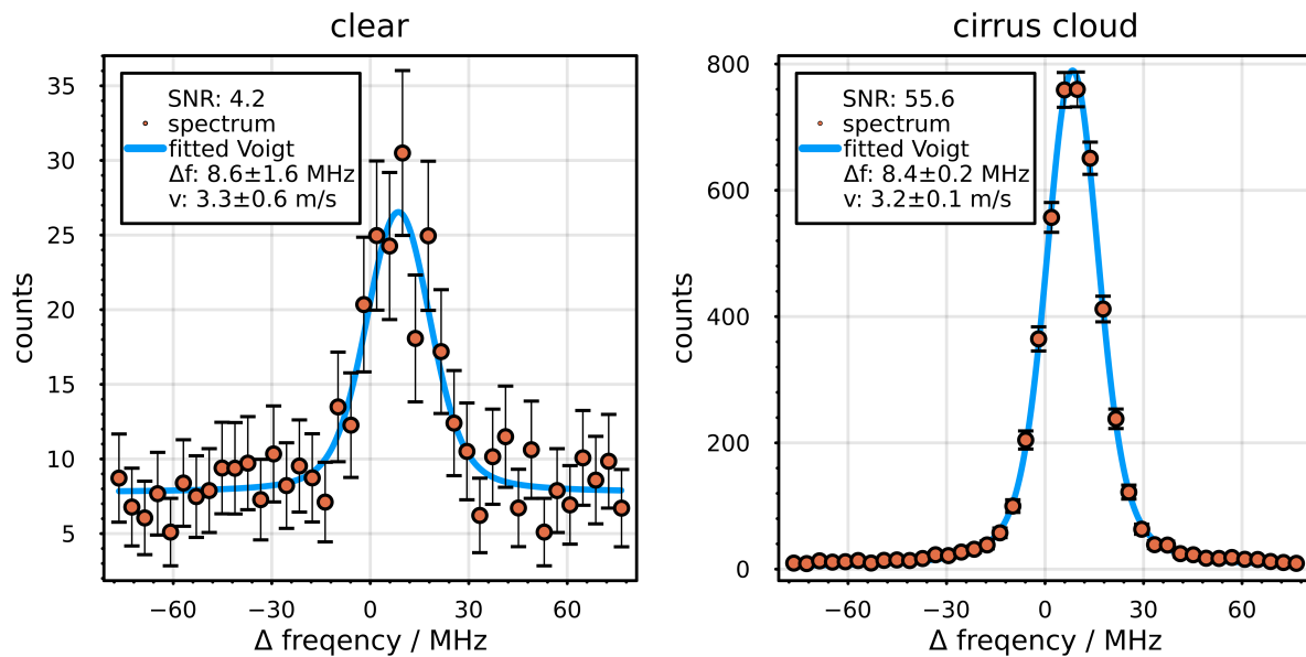
Figure 5. Example of the spectrum measured from 9.25 km to 10.25 km in the north field of view, together with the fitted Voigt function in clear air (left) and in a cirrus cloud (right). Corresponding signal-to-noise ratios and errors in frequency offset and winds derived from the fits are shown in the inlets.
