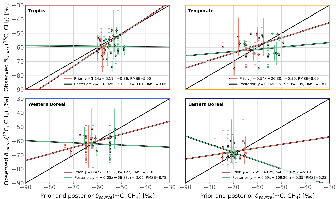
Figure B2. Comparison between prior-posterior and observed wetlands \delta_{source}(^{13}\text{C}, \text{CH}_4) . Observations are taken from the Supplementary Data 1 provided by Oh et al. (2022). For each observation, prior and posterior values are sampled using the gridcell corresponding to the latitude and longitude provided in the dataset. Error bars for each observation point represent the observation uncertainty. Each panel shows a comparison with observations located in a selected region: Tropics ( <30^\circ\text{N/S} ), Temperate ( 30\text{--}50^\circ\text{N/S} ), Western Boreal ( 50\text{--}90^\circ\text{N} and <15^\circ\text{W} ) and Eastern Boreal ( 50\text{--}90^\circ\text{N} and >15^\circ\text{W} ). For each panel, the identity line and two linear fitting lines (prior in green and posterior in red) are displayed. The parameters of the fitting lines, the Pearson's correlation coefficients ( r ) and the root-mean-square error (RMSE) are given in the legend box.
