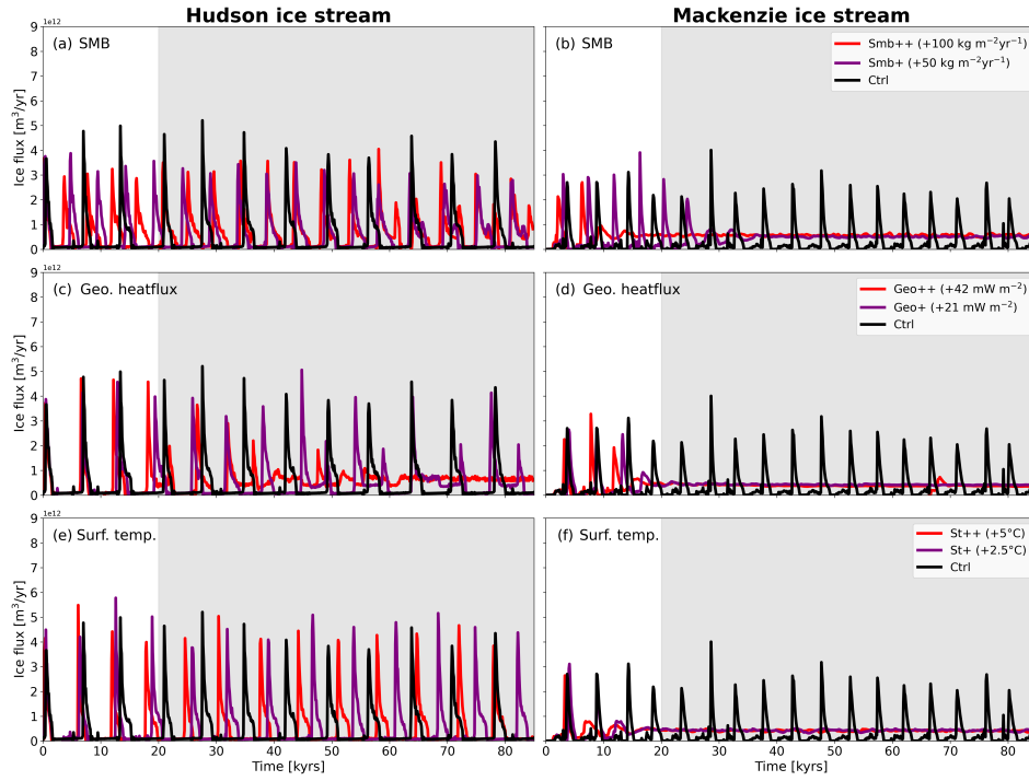
Figure B1. Similar to Fig. 7 but only shows the positive perturbation experiments where additional intermediate scenario simulations were performed. The panels show response to (a,b) SMB, (c,d) geothermal heatflux, and (e,f) ice surface temperature. Grey shading highlights analysis period.
